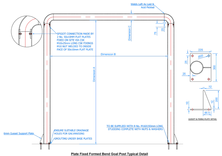
Plate Fixed Formed Bend Goal Post Typical Detail
