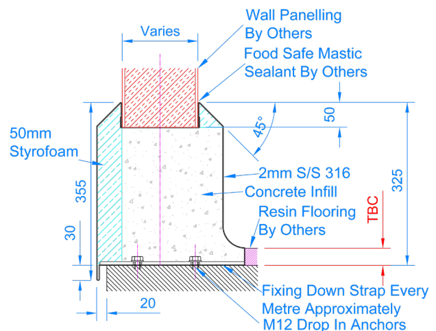
AQB4 - External Insulated Kerb Scale -1:8
