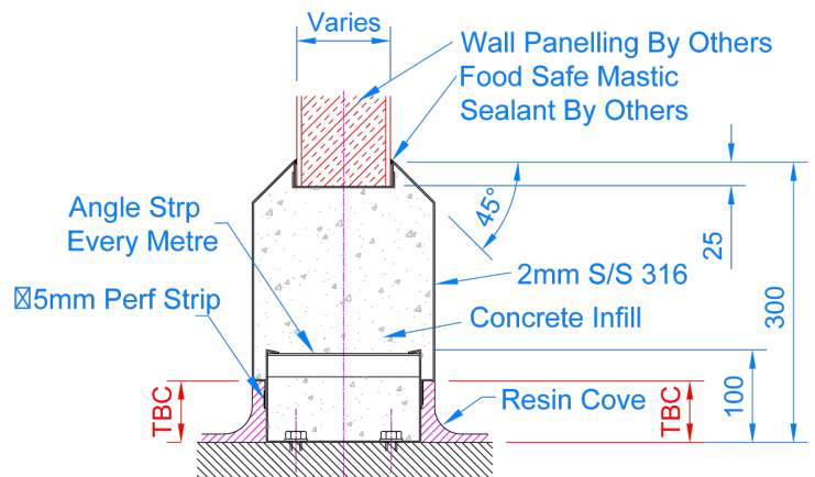
AQA2 Double Sided Kerb Scale -1:8
