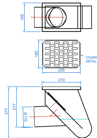
Aqualine Trent Gully \varnothing 110mm Side Outlet Scale - 1:5
