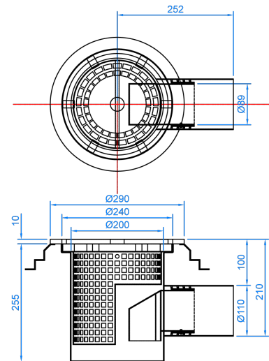
Aqualine Medway Gully Round Top \varnothing 110mm Side Outlet Scale - 1:5
