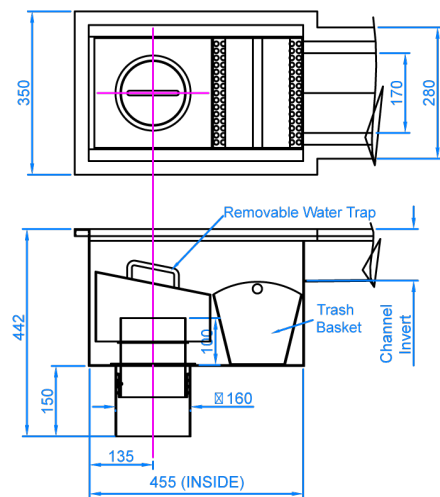
Avon Outlet 170mm End Bottom \varnothing 160mm Outlet Scale -1:8
