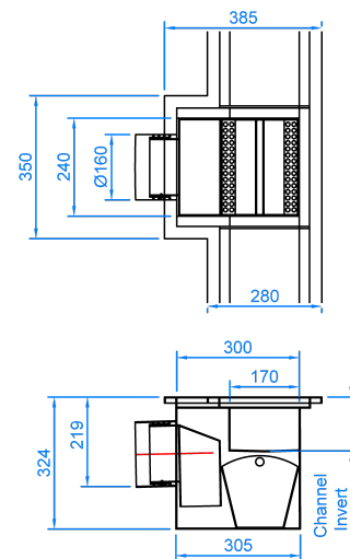
Avon Outlet 170mm Central Side \varnothing 160mm Outlet Scale -1:8
