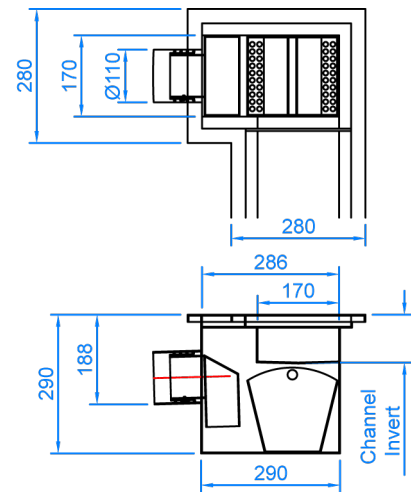
Avon Outlet 170mm End Side \varnothing 110mm Outlet Scale -1:8
