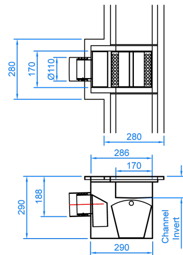
Avon Outlet 170mm Central Side \varnothing 110mm Outlet Scale -1:8
