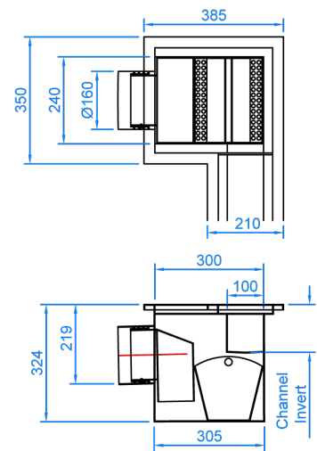
Avon Outlet 100mm End Side \varnothing 160mm Outlet Scale -1:8
