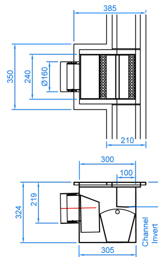
Avon Outlet 100mm Central Side \varnothing 160mm Outlet Scale -1:8
