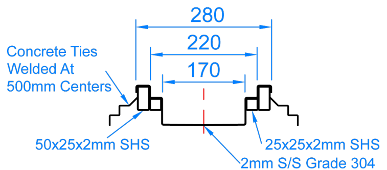
AQUALINE HEAVY DUTY 170mm DRAIN CHANNEL SECTION SCALE -1:8
