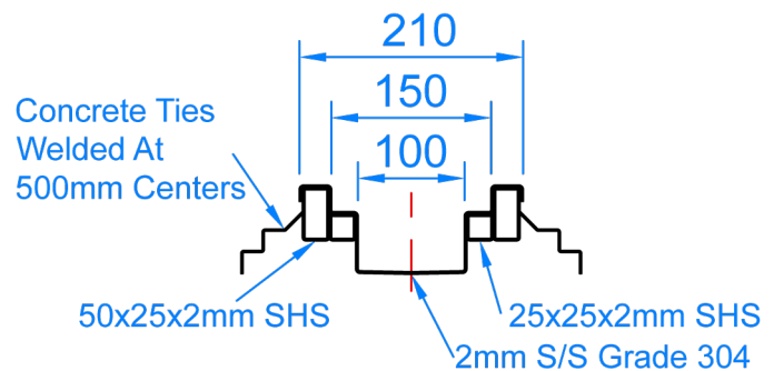
AQUALINE HEAVY DUTY 100mm DRAIN CHANNEL SECTION SCALE -1:8
